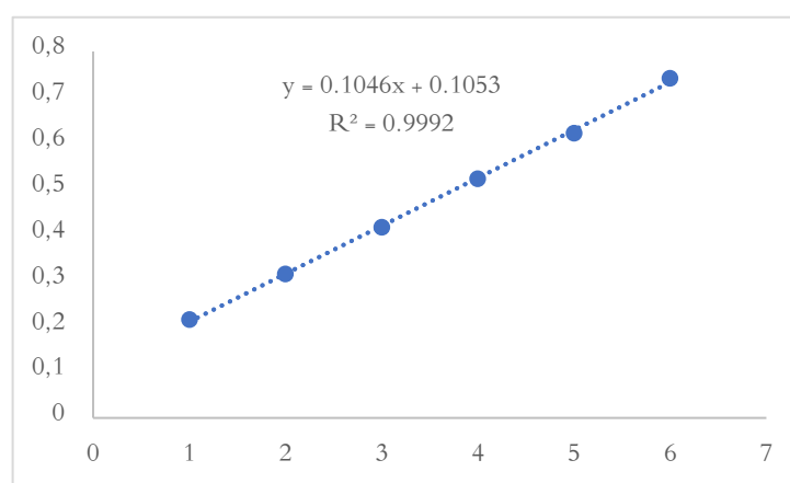
Figure 3. Linearity Curve of Rhodamine Standard
